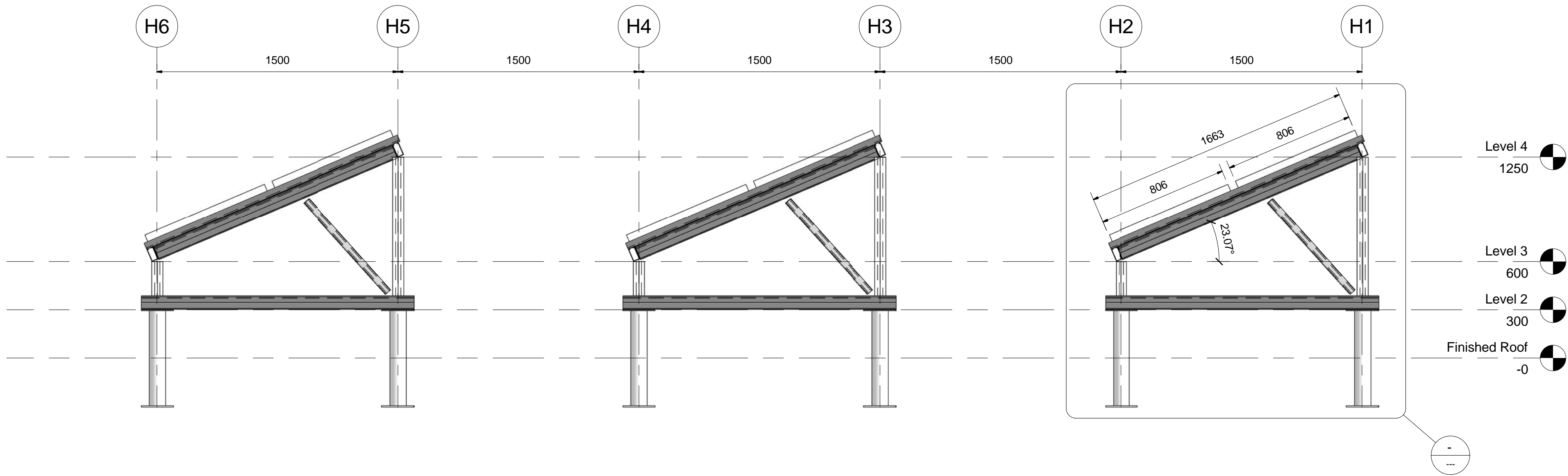
1 Partial East Elevation 1 : 20
