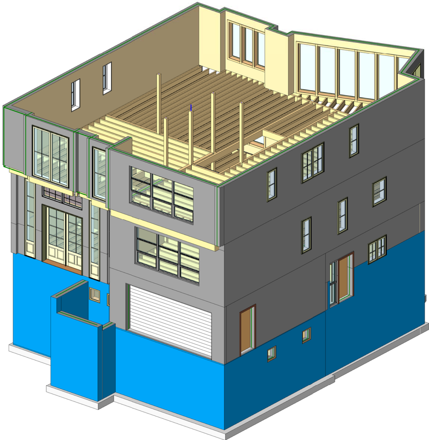
① Cover Page Isometric View
